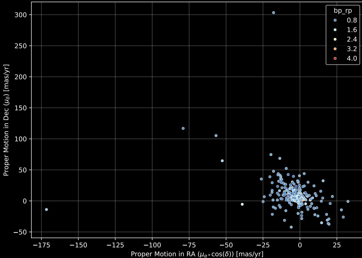
GALAH DR4 Field: [7166] Proper Motion Diagram (n= 248)
