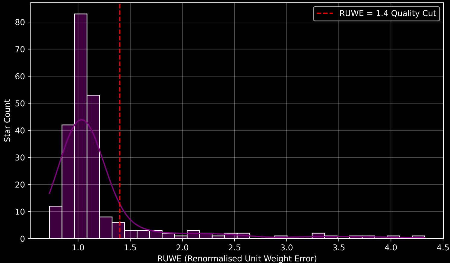
GALAH DR4 Field [7166] RUWE Distribution (n= 234)
