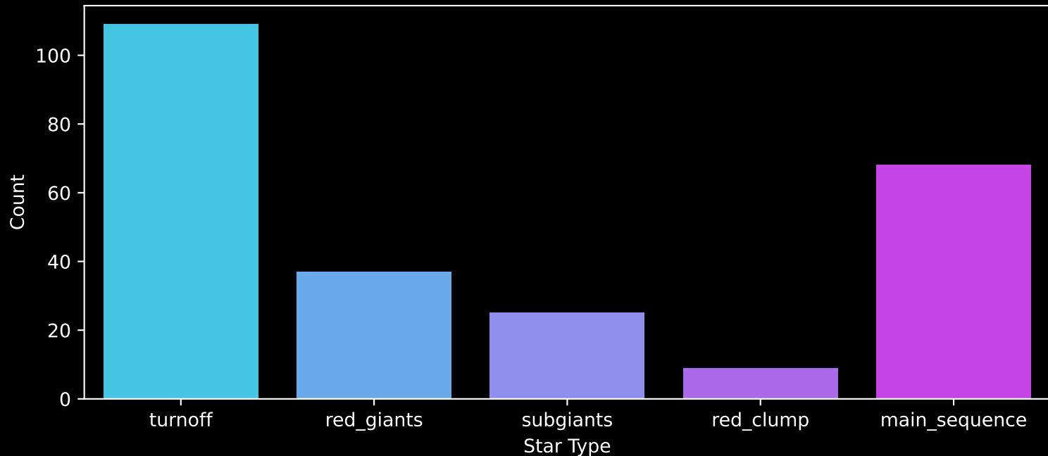
GALAH DR4 Field: [7166] Count plot of Star Type
