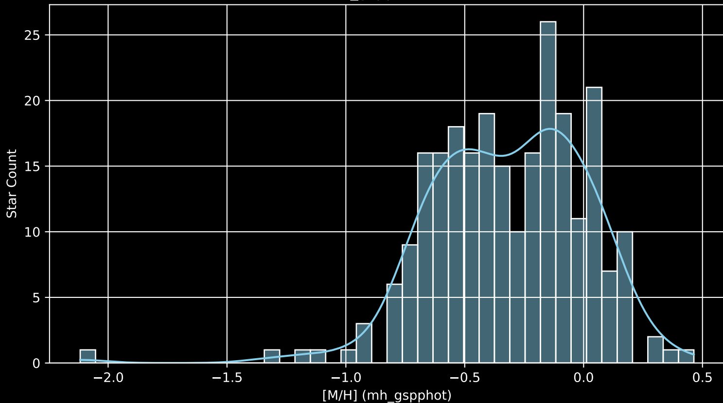
GALAH DR4 Field: [7166] [M/H] (mh_gspphot) (n= 247)
