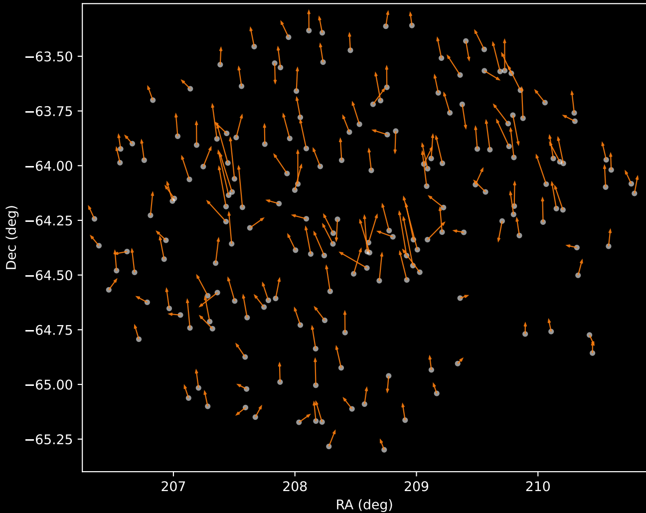
GALAH DR4 Cluster 2 Proper Motion Vectors (n=184)
